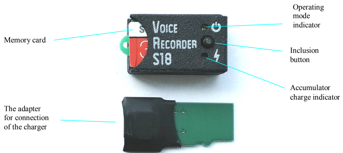
Fig. 2. Appearance of voice recorder Soroka-18E
